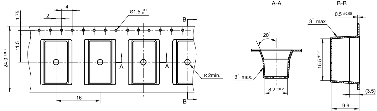
Tape Dimensions (S1 type: Short terminal SMT)
