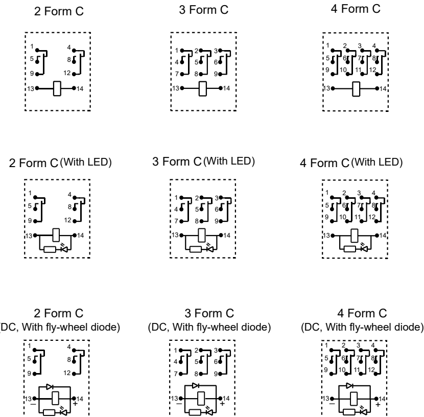
Wiring Diagram (Bottom view)
