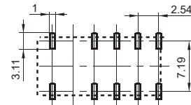
2 coils latching
