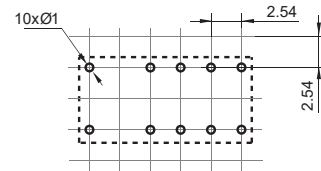
2 coils latching
