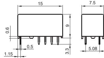
2 coils latching
