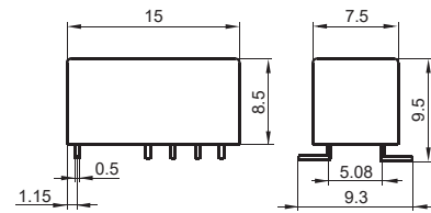
2 coils latching
