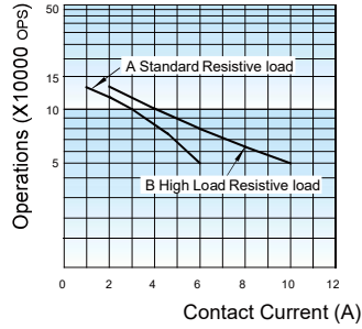
ENDURANCE CURVE
