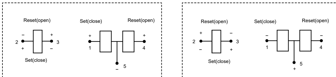
Standard polarity
