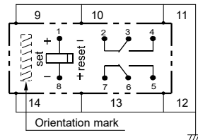
Reset condition
