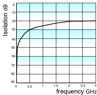
Isolation (between open contacts)
