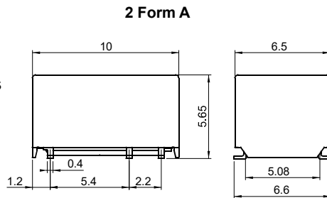
Outline Dimensions Short terminal SMT type
