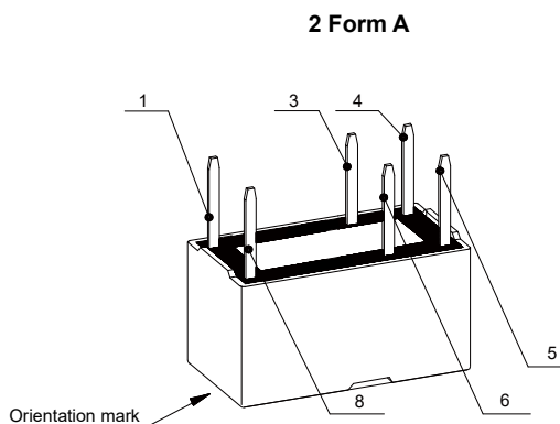
Pin Layout
