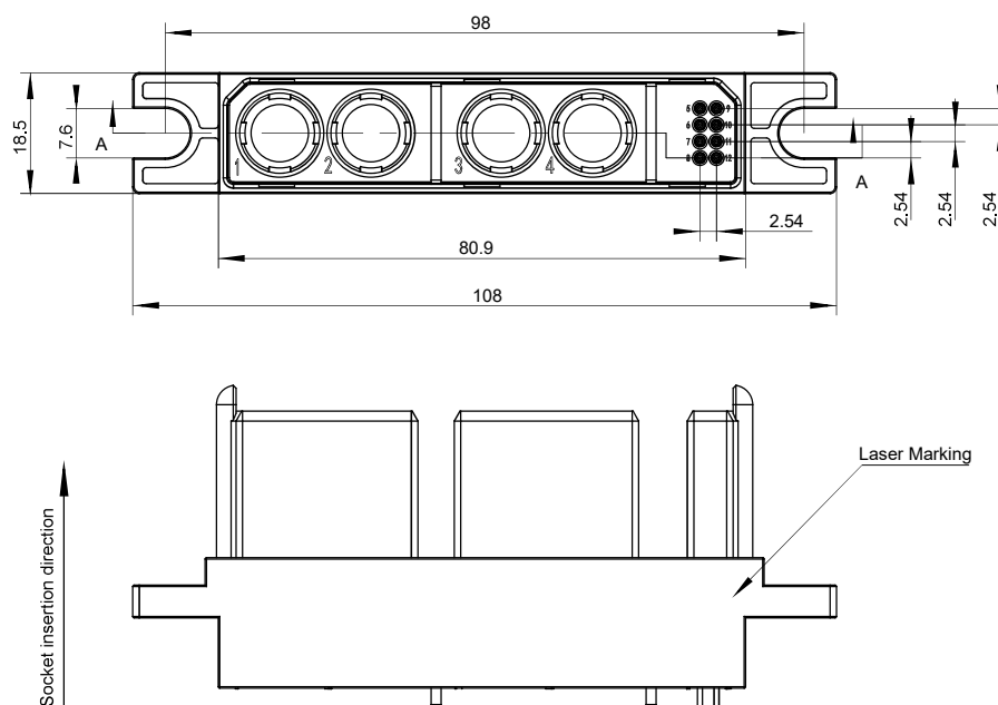
Outline Dimensions
