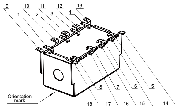
Pin Layout (Single side stable & 1 coil latching)
