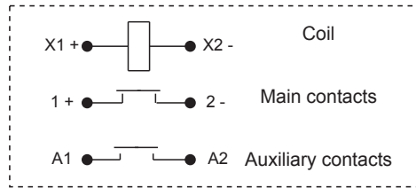
Wiring Diagram
