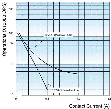
ENDURANCE CURVE
