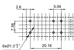
1 Form B
