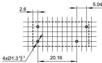
1 Form A
