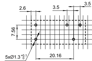
1 Form C
