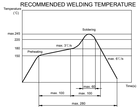
REFLOW WELDING, TEMPERATURE ON PCB BOARD
