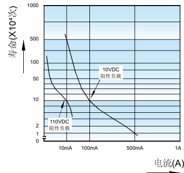
ENDURANCE CURVE
