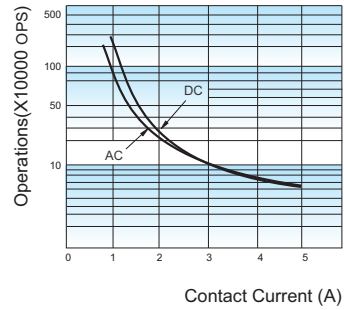
ENDURANCE CURVE
