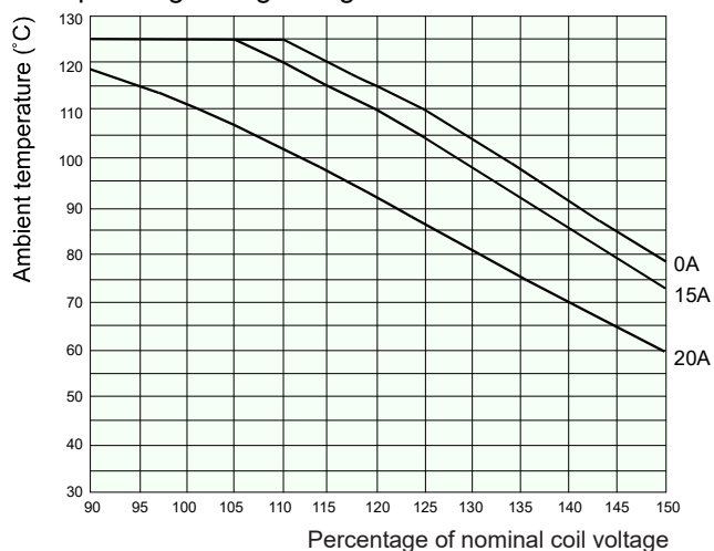
Ambient temp. curve (one cycle)
