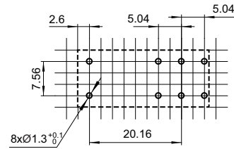
1 Form C
