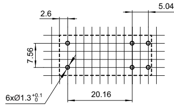
1 Form A
